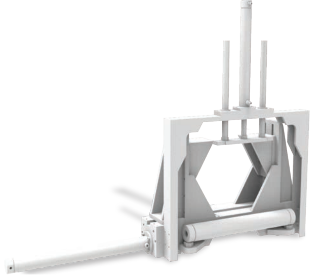
KURTAĞZI - ÜSTBASKI DOVETAIL CLAMPING - BUNDLE CLAMPING
